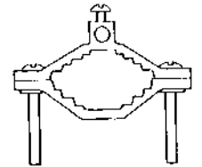
Figure 6 - Clamp for 5/8-inch thick rod
