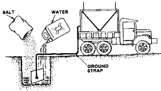
Figure 11 - Grounding plate installation
