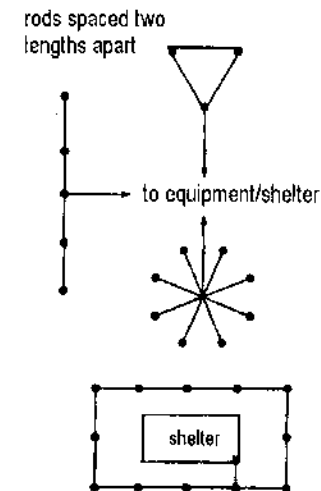
Figure 13 - Typical ground rod configurations
