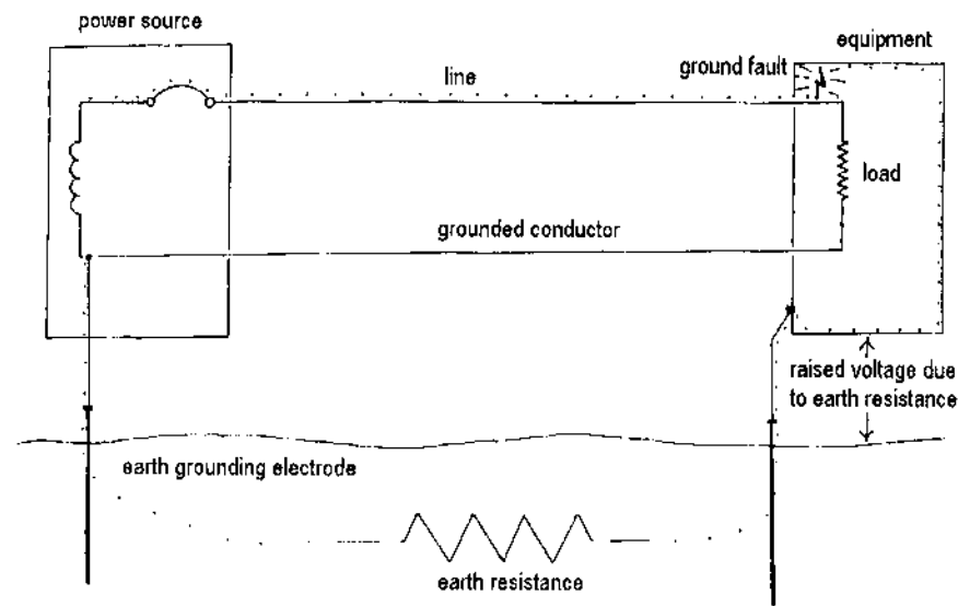
Figure 25 - Soil provides a poor impedance path; circuit breaker will not trip.
