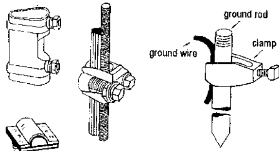
Figure 3 - Examples of suitable clamping devices
