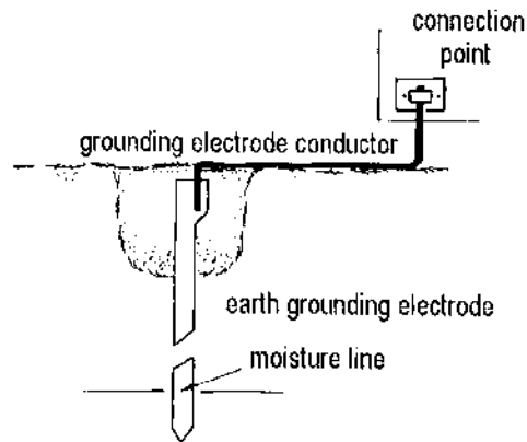
Figure 2 - Key elements of an earth grounding system
