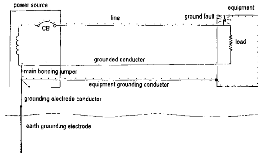
Figure 23 - Low impedance path provided by the EGC during a fault
