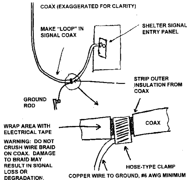
Figure 22 - Expedient signal entry protection
