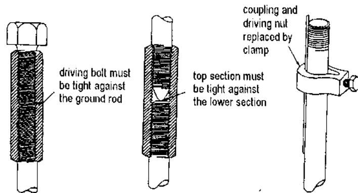
Figure 10 - Ground rod components and assembly
