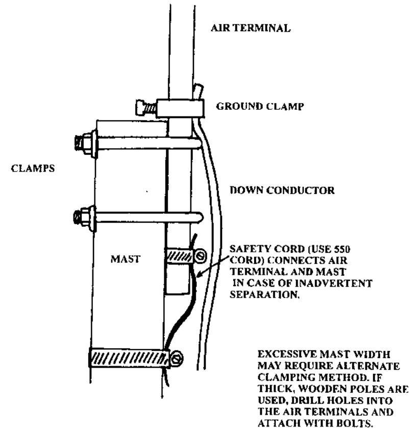
Figure 18 - Detail #1
