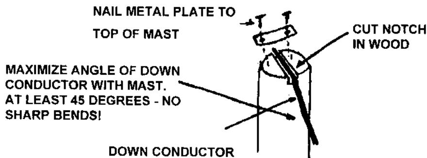
Figure 20 - Detail #2
