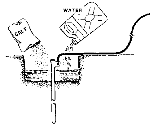
Figure 12 - Treatment of soil
