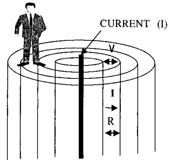
Figure 26 - Step potentials
