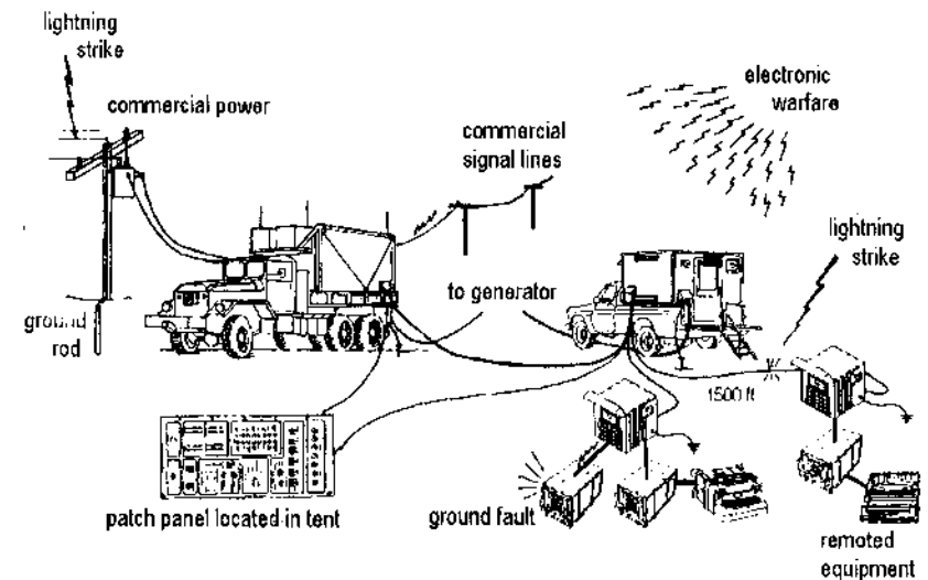
Figure 24 - Complex systems can have multiple sources and paths for faults
