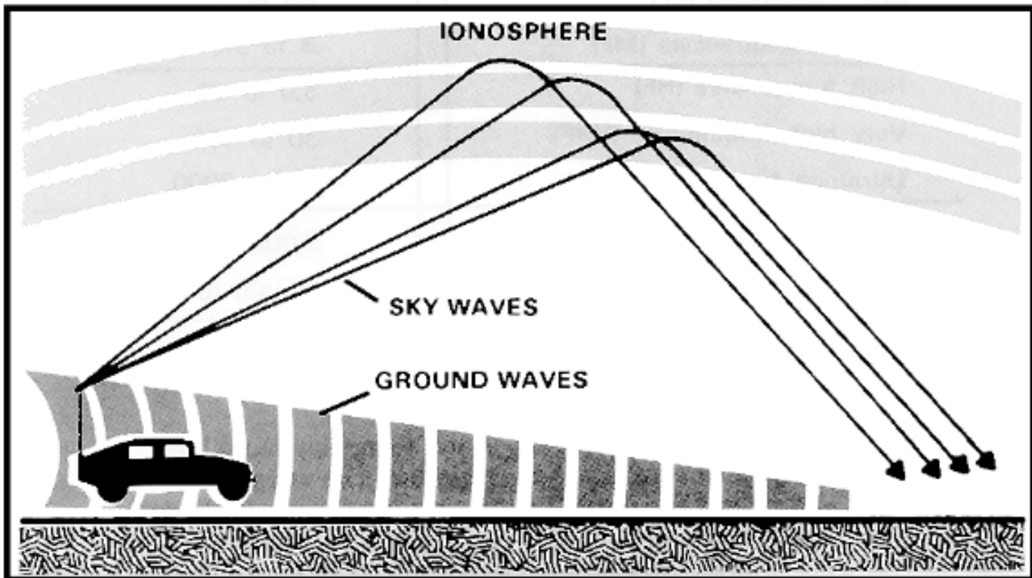
Figure 2-11. Principal paths of radio waves.
