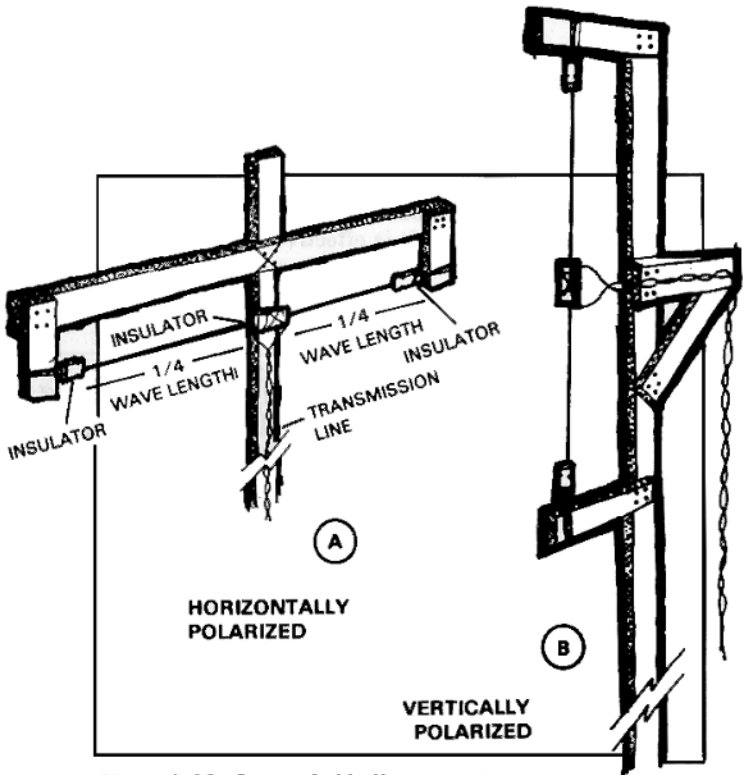
Figure 3-33. Center-fed half-wave antenna.
