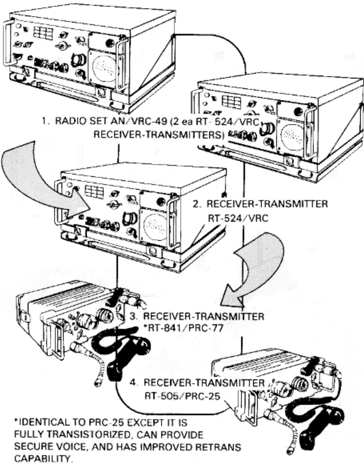
Figure F-3. Radio equipment.
