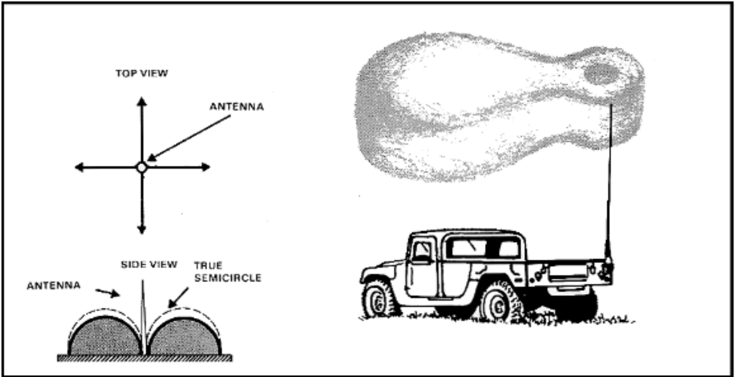
Figure 3-15. Radiation pattern of a whip antenna.
