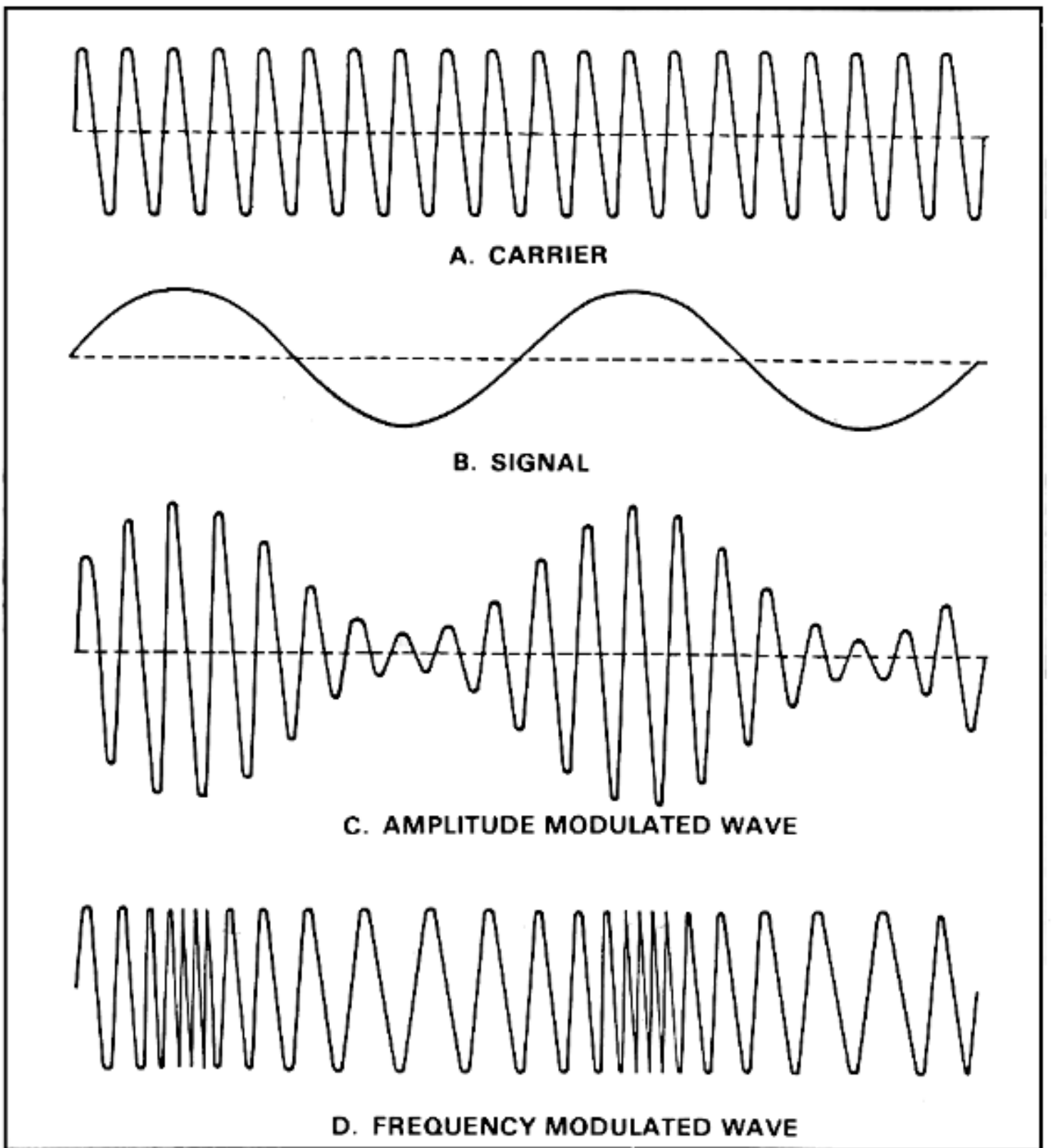
Figure 2-17. Wave shapes.
