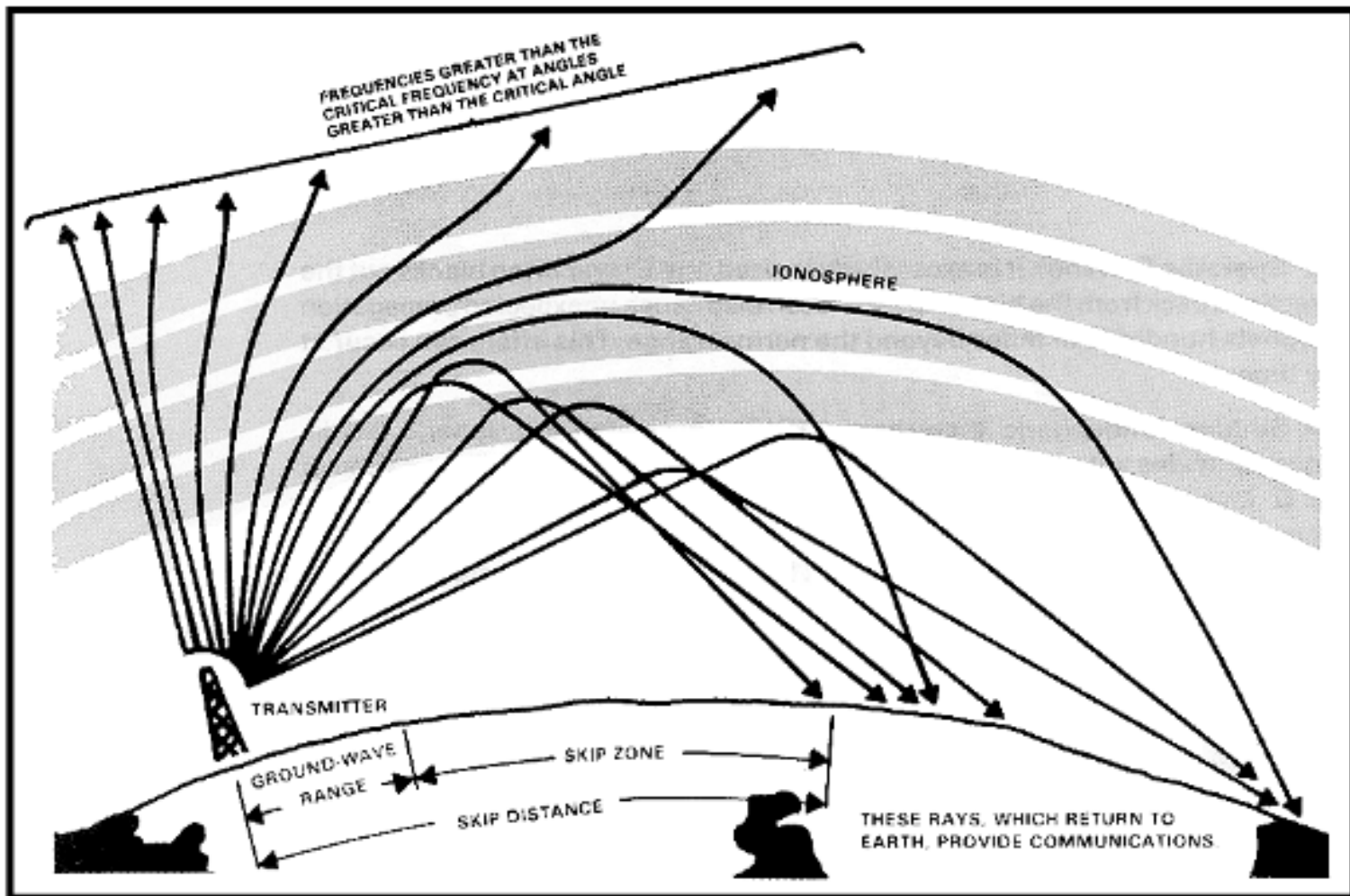
Figure 2-14. Sky wave transmission paths.
