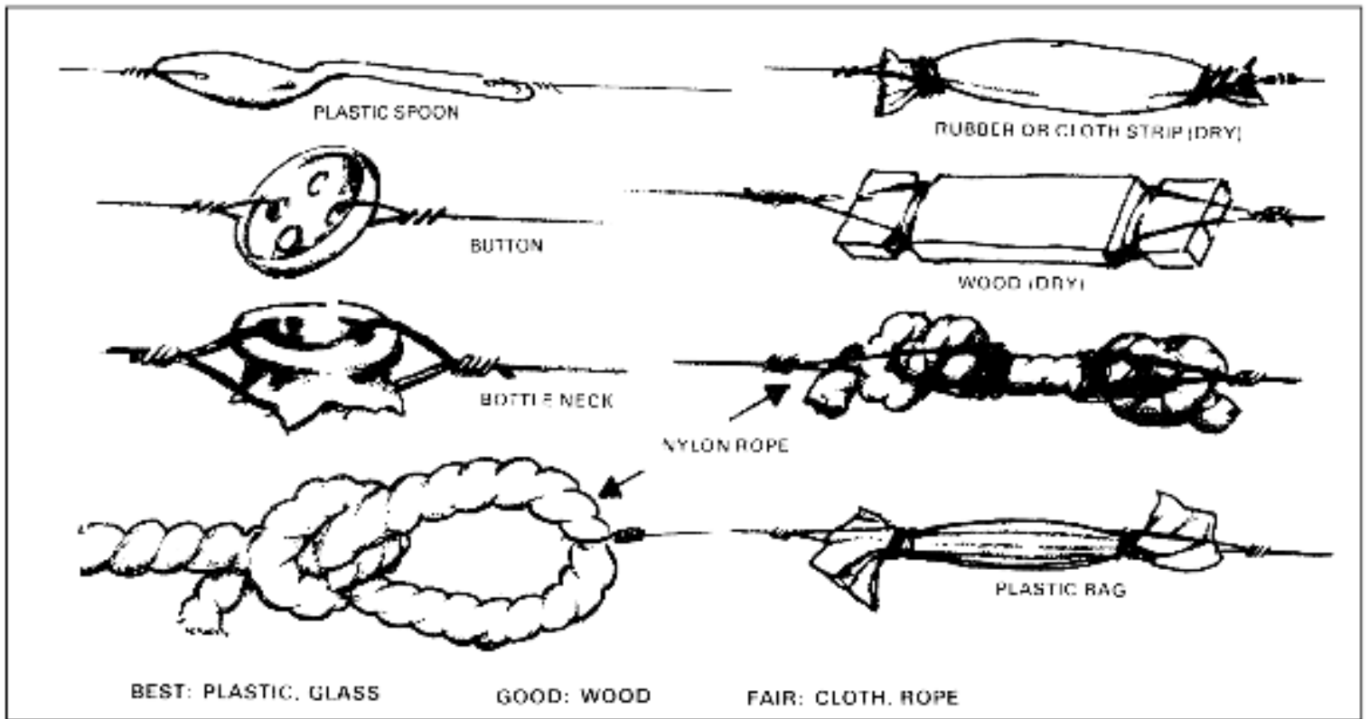
Figure 3-26. Improvised insulators.
