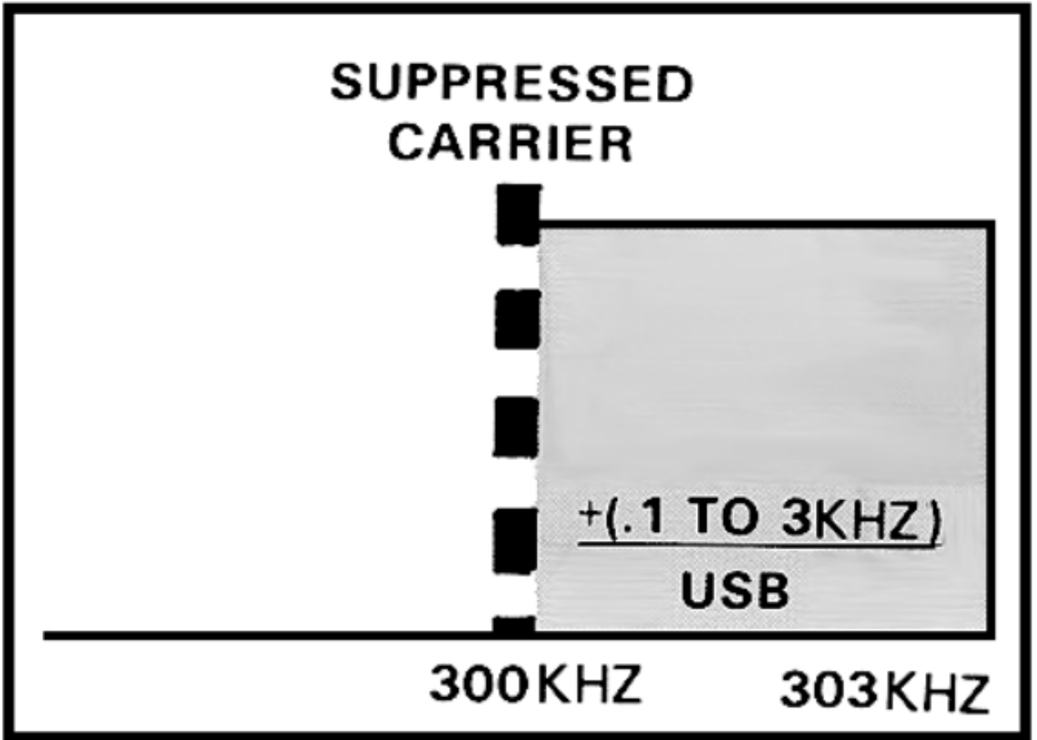
Figure 2-19. Single-sideband system.
