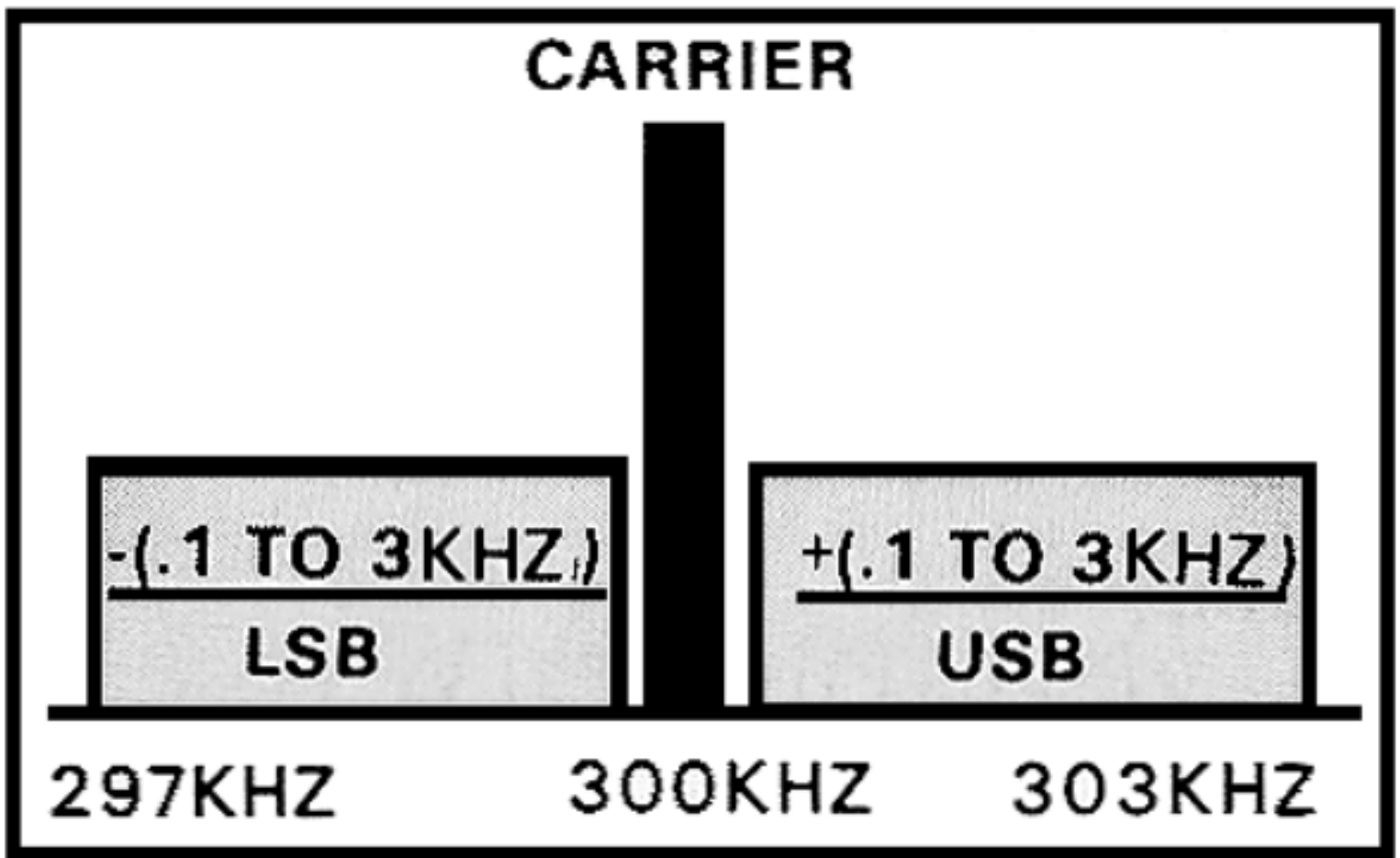
Figure 2-18. Amplitude-modulated system.
