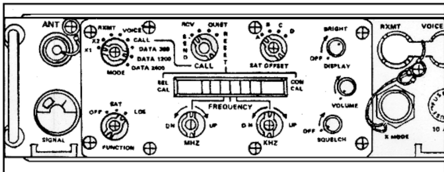
Figure L-5. Receiver/Transmitter RT-1402(G).
