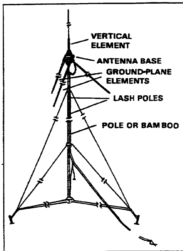
Figure 1-7. RC-292 ground-plane antenna
